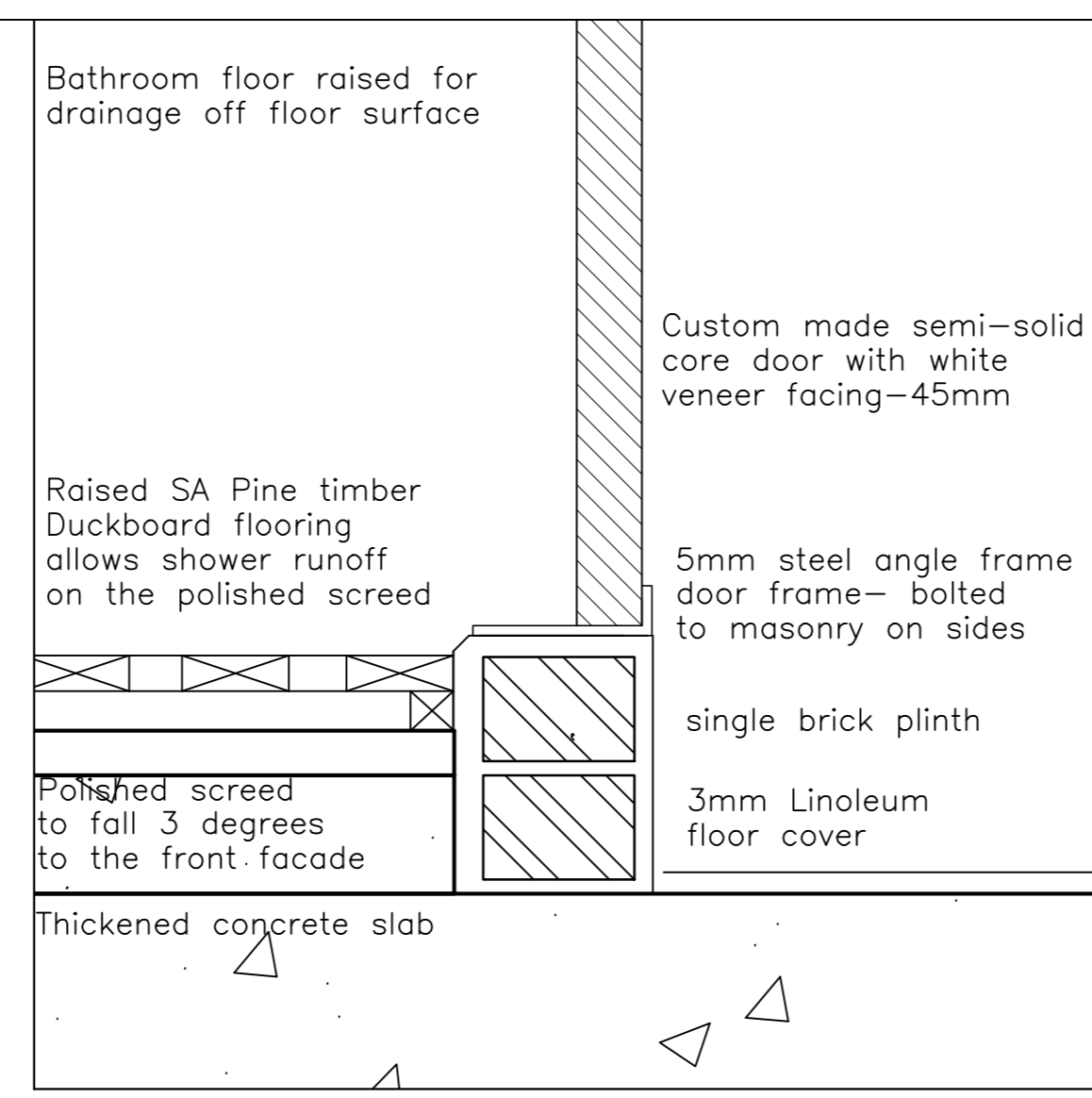
DETAIL C 1:5
