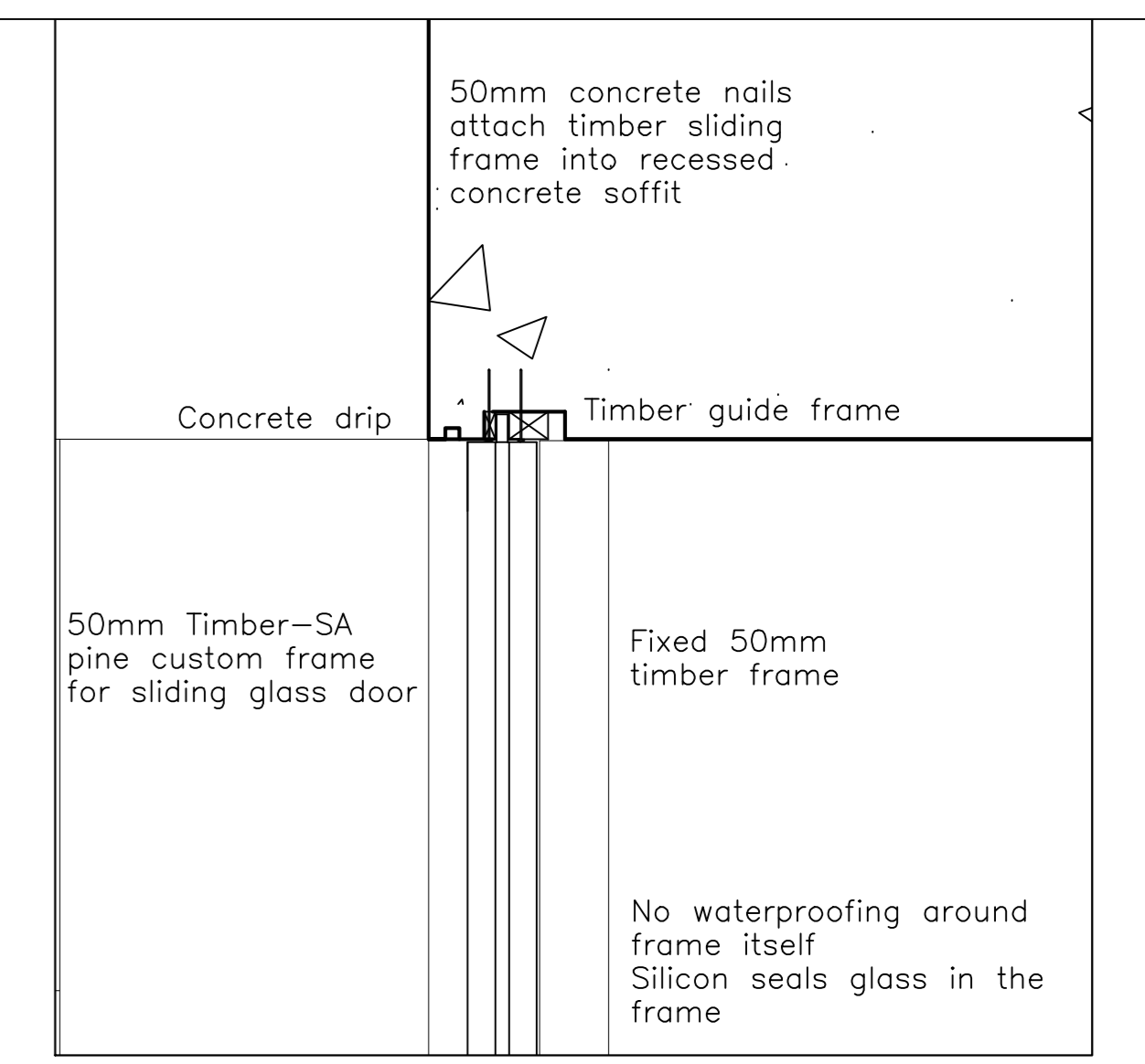
DETAIL F 1:5
