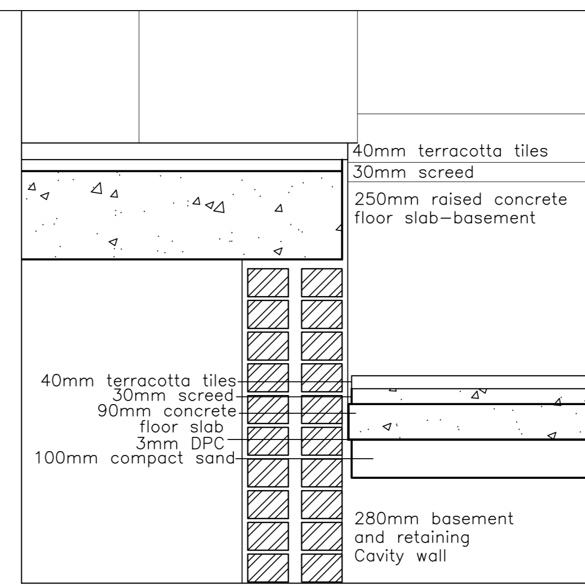
DETAIL D 1:10
