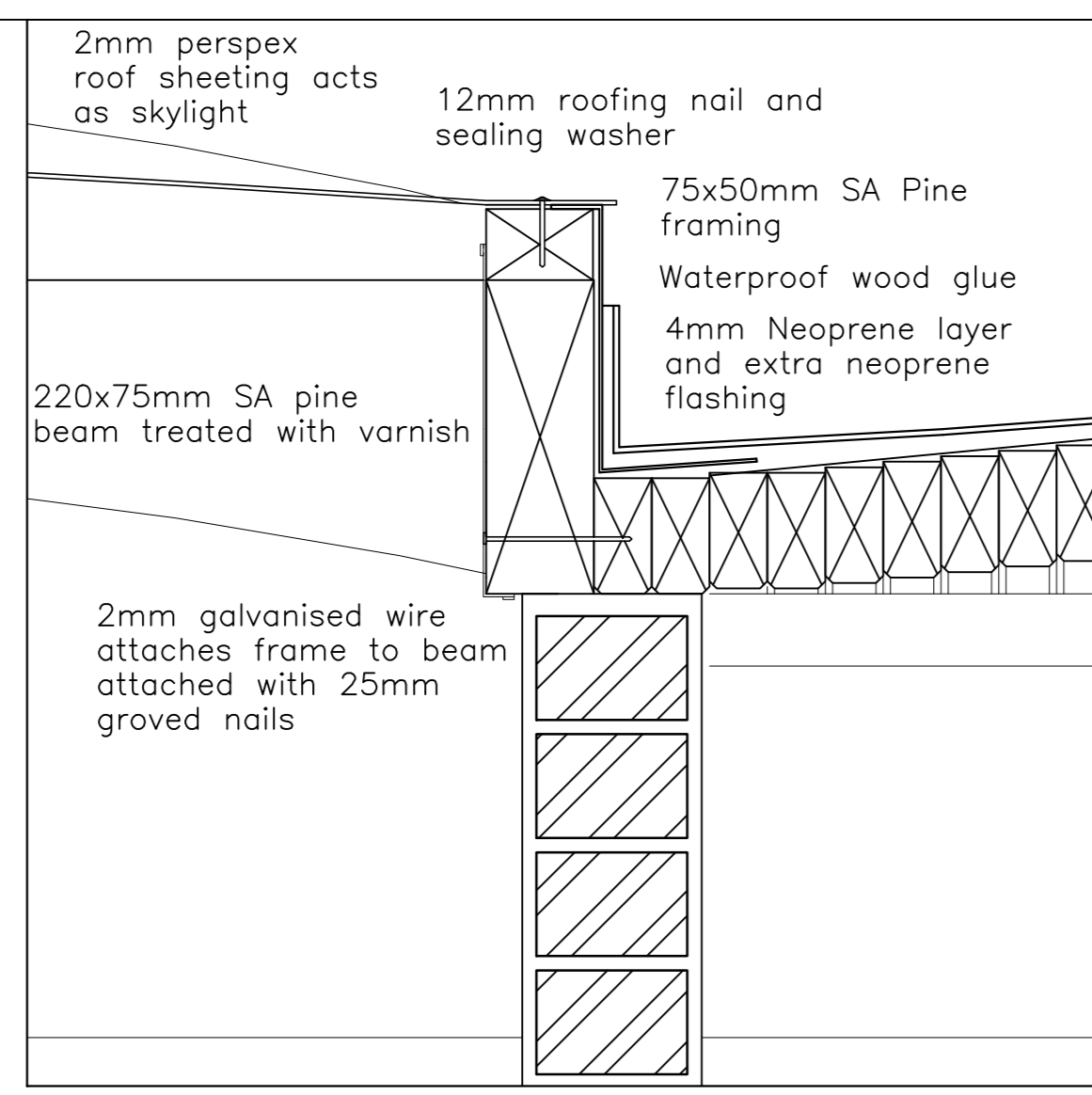
DETAIL B 1:5
